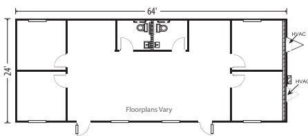
24' x 64' Building w/ Restroom* – Item 1949
