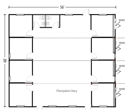
48' x 56' Building w/ Restroom* – Item 1743
